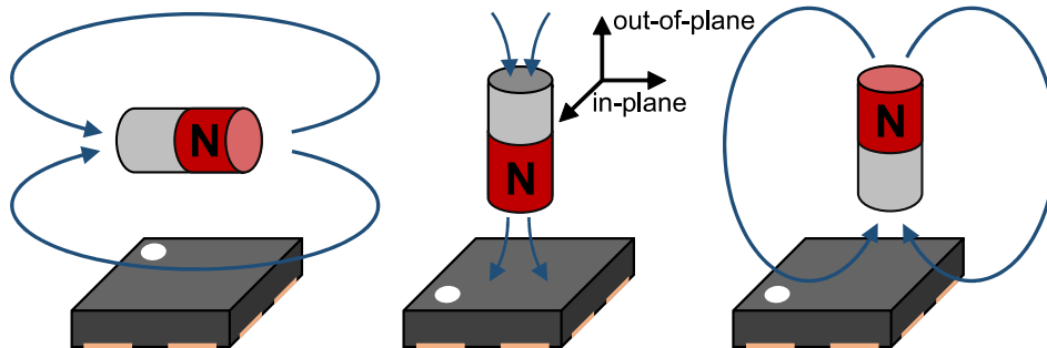
Figure 1. ADK991 sensor direction of magnetic sensitivity.
